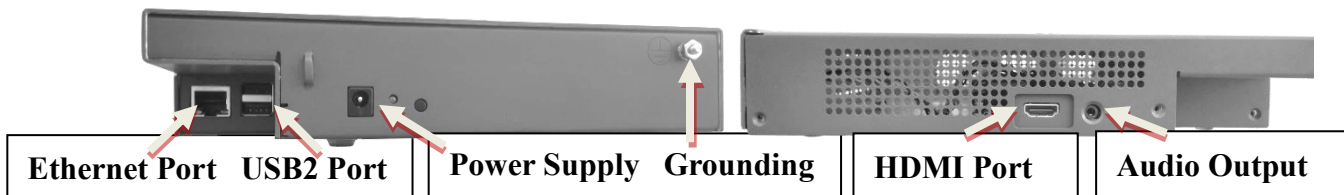
Figure 1: Ethernet & USB2 ports, power supply and grounding screw on Spark CXS1000 rear panel; HDMI and audio ports on Spark CXS1000 side panel.
